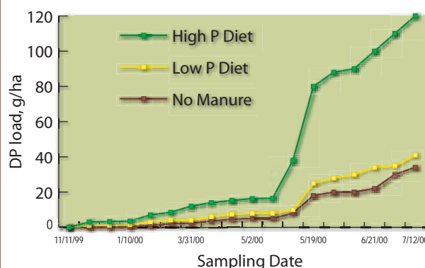
Figure 16. Cumulative dissolved phosphorus (DP) load in natural runoff from manures differing in P content.
